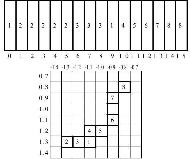
Fig. 4. Final segmented liner for 1500 Hz. Global attenuation = 33.5 dB.
